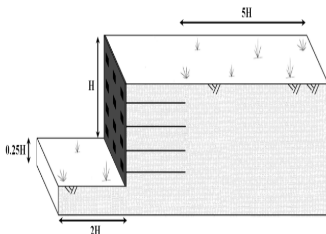
Figure-3 Dimensions of constructed models
