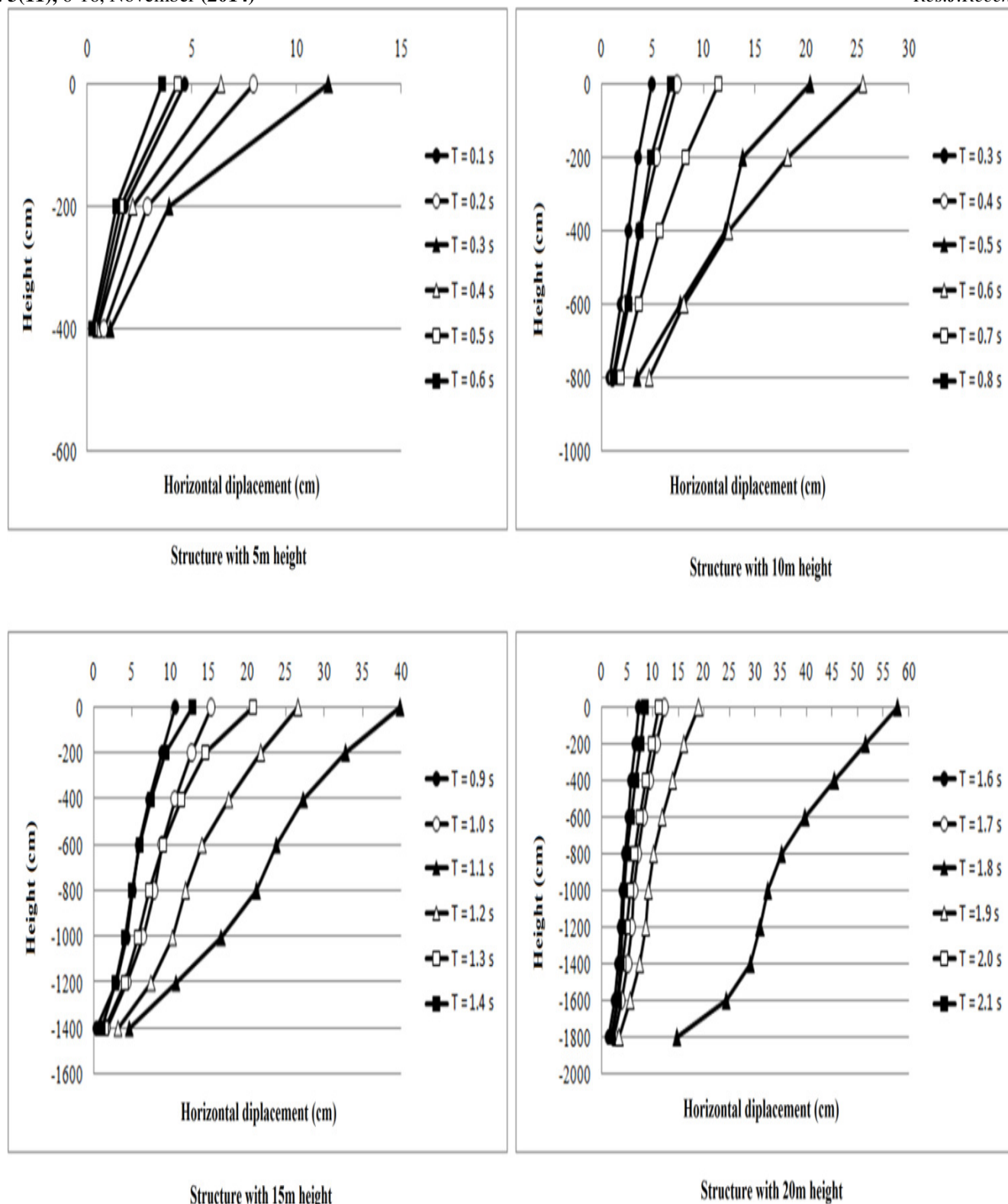
Figure-9 Seismic performance of soil nailing system in the form of horizontal displacement against loading period
