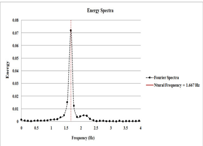
Energy spectrum for structure with 10m height
