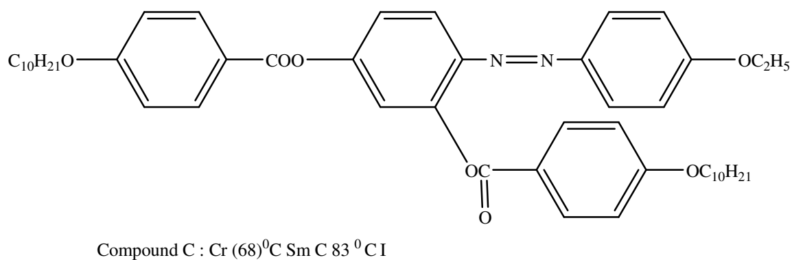
Figure -2 The comparative molecular structures and transition temperatures of compound 9, A, B and C
