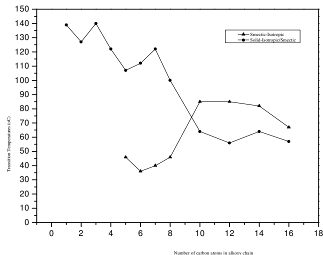
Figure-1 The plot of transition temperatures versus number of carbon atoms in alkoxy chain
