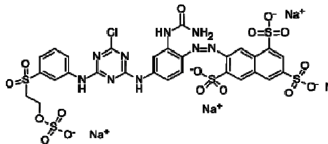
C.I. Reactive yellow 145
