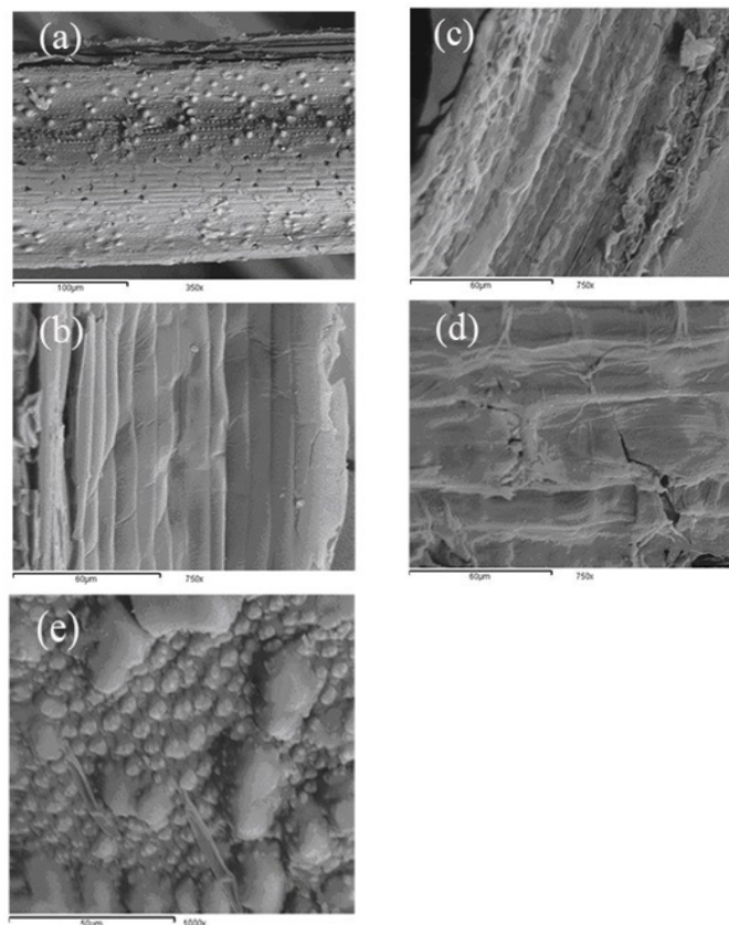
Figure-2 SEM micrographs of original RS (a), PE 3 -coated RS (b), PE 4 -SiO 2 -coated RS (c), PE 5 -coated RS (d), and PE 6 -SiO 2 -coated RS (e)
