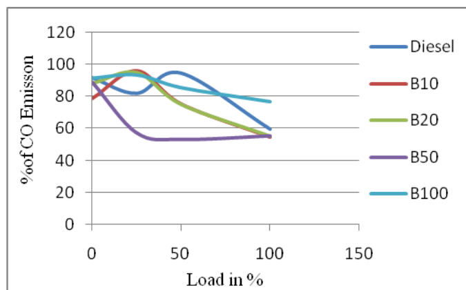
Figure-1 CO emissions for diesel and Karanja biodiesel fuel
