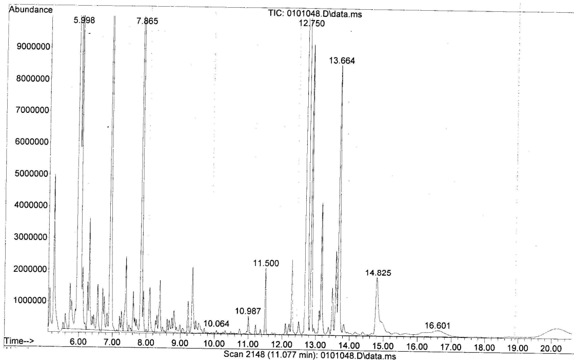
Figure-1 Gas chromatography (GC) spectrum of hyptis spicigera
