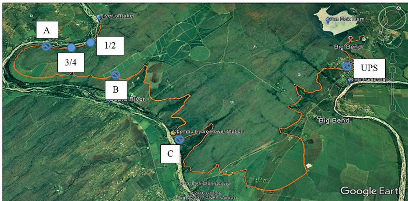
Figure-1: Layout of the USL main gravity earth canal and its physical attributes, ● = scour gates, ◻ = flumes.
