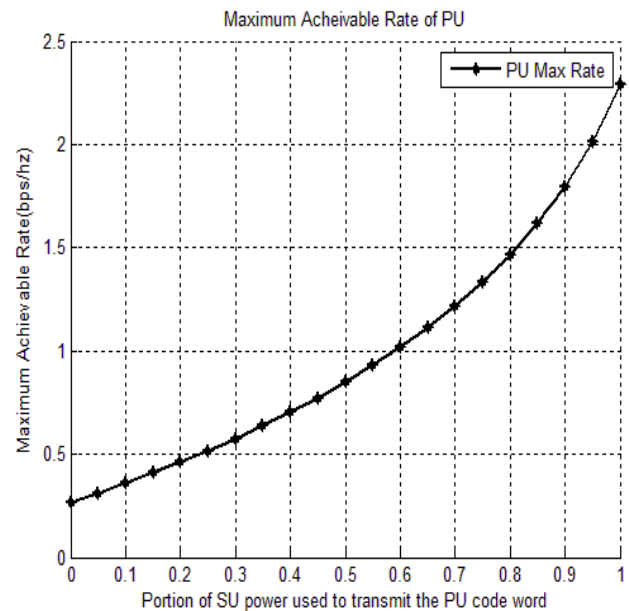
Figure-2 Achievable PU rate (Bits/sec/Hz) Vs Portion of SU power ( \gamma ) to transmit PU codeword
