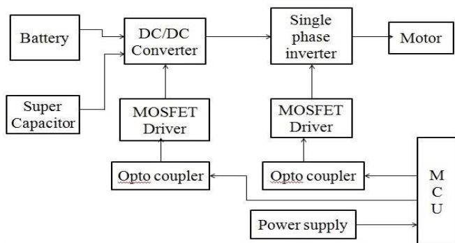
Figure-1: Hybrid energy storage system for electric vehicle 2 .
