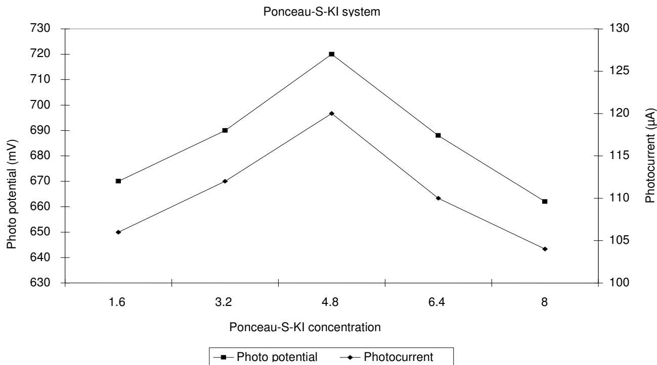
Figure-3 Variation of photo potential and photocurrent with KI concentration
