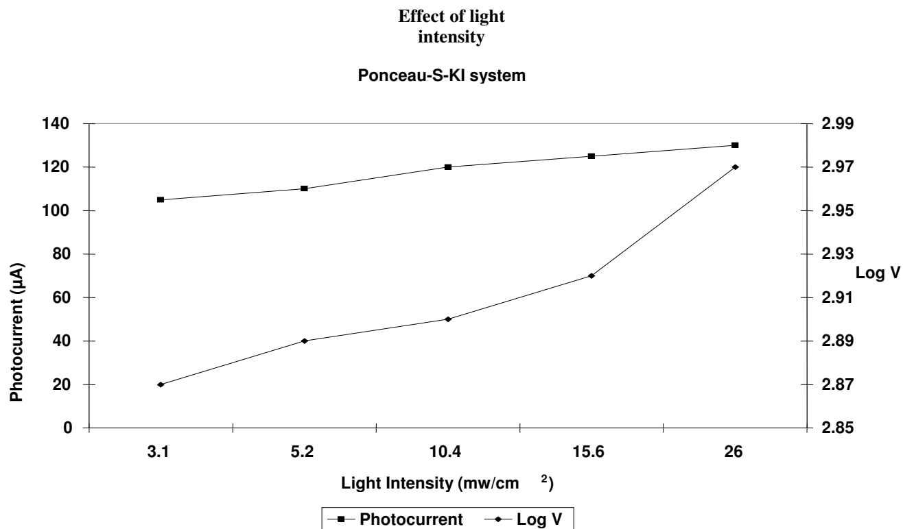
Figure-4 Variation of photopotential and photocurrent with light intensity Ponceau-S-KI System
