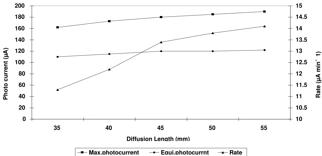
Figure-5 Variation of current with diffusion length
