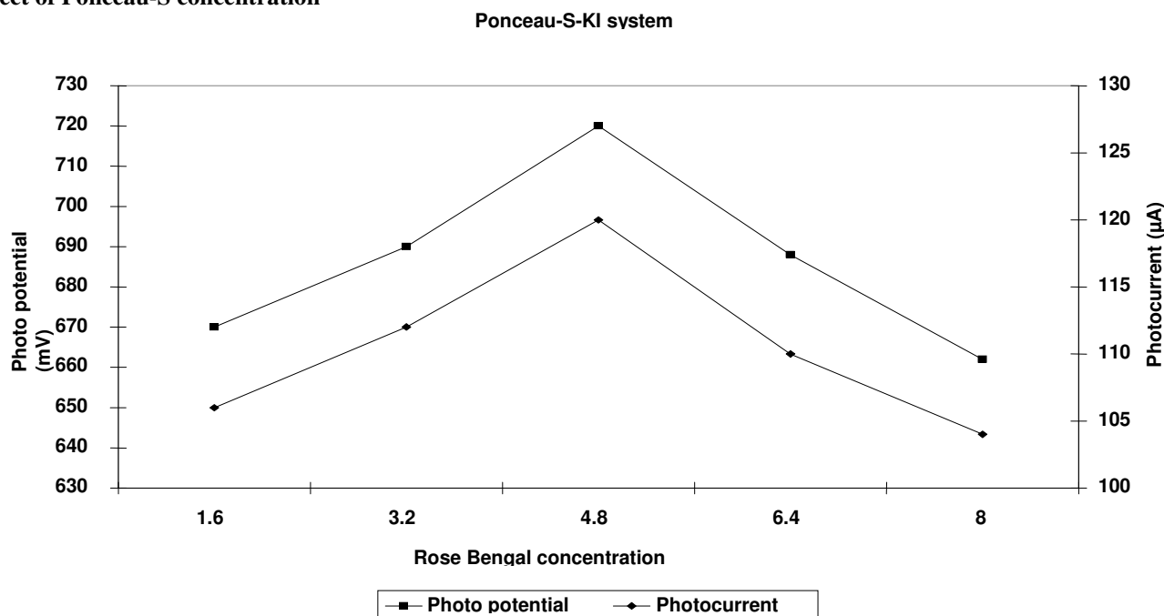
Figure-2 Variation of photopotential and photocurrent Ponceau-S concentration
