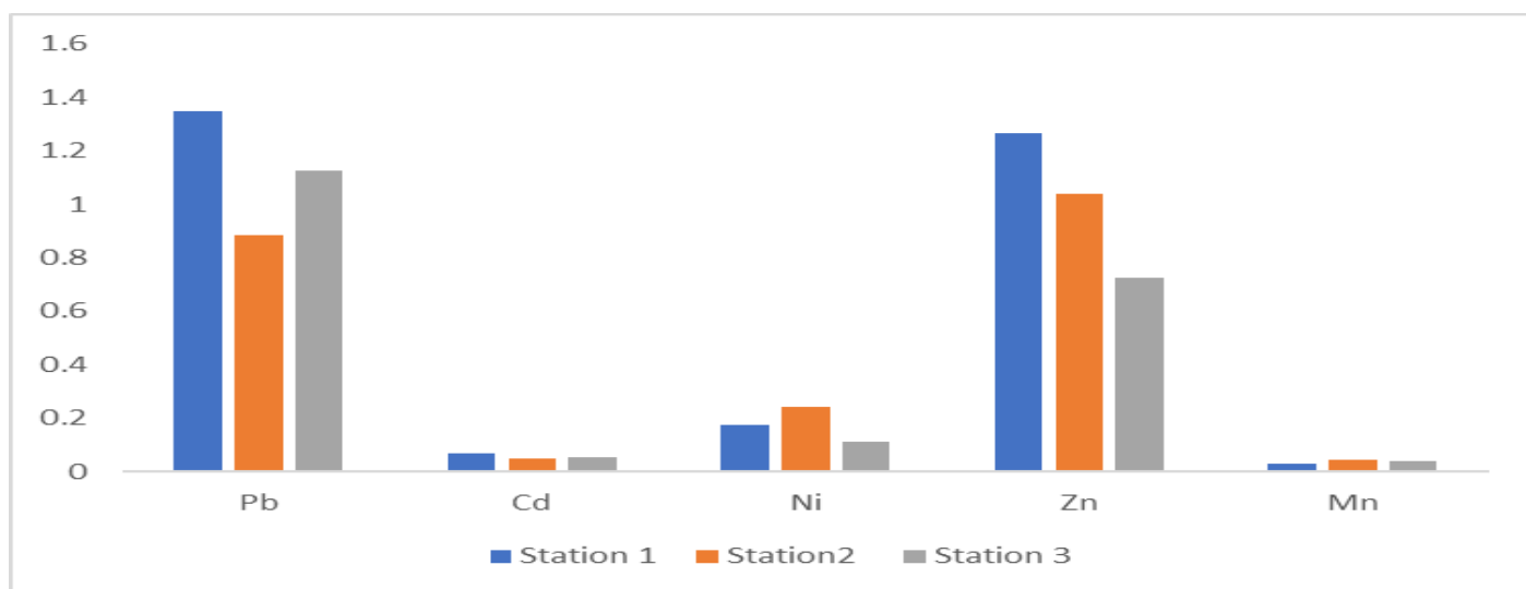
Figure-2: Heavy Metals in the Sediments of the River Nun Estuary.
