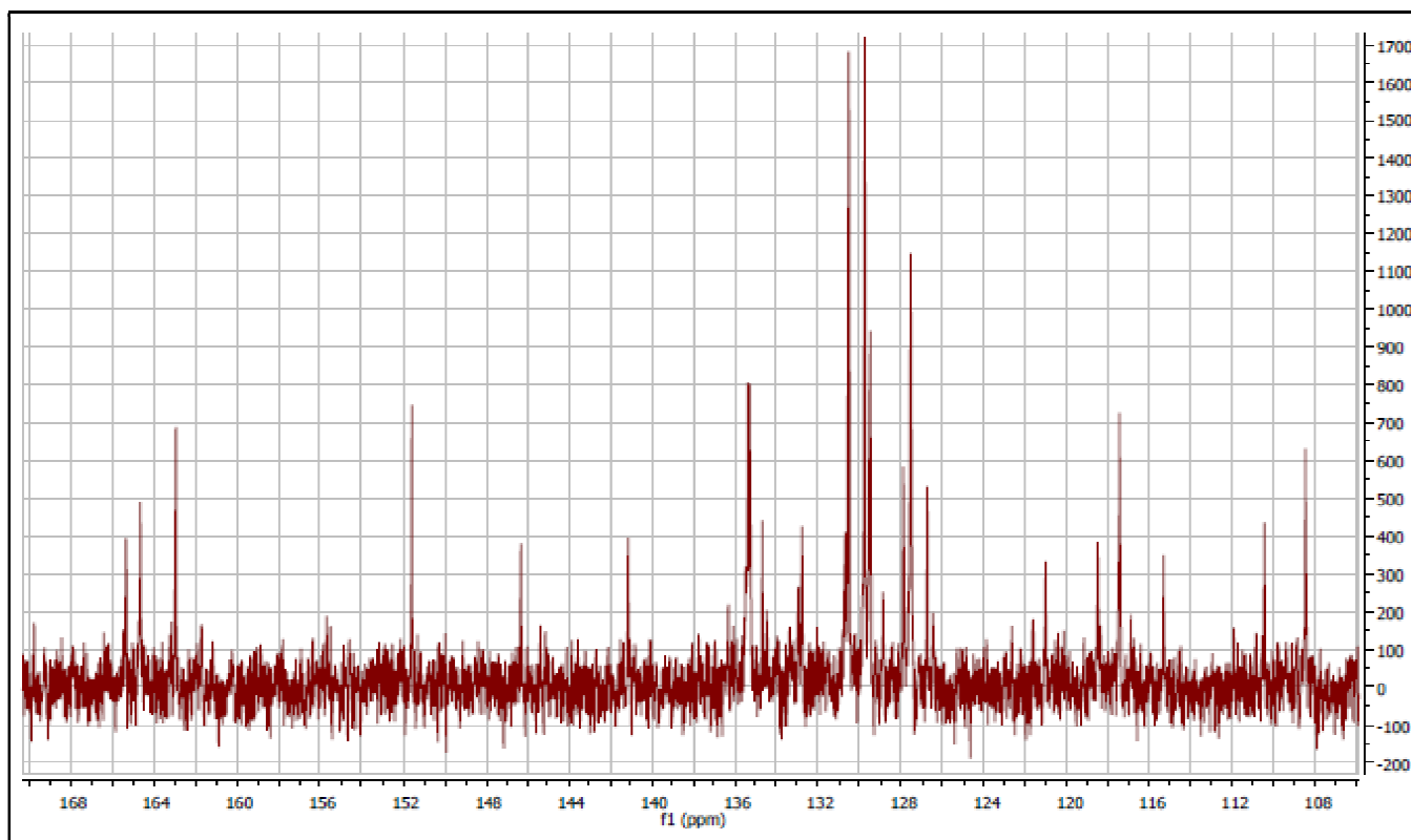
Figure-3: Absorption Spectra of TBPO.
