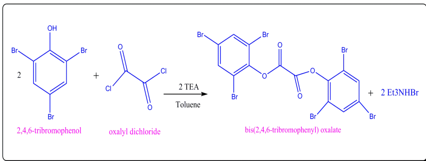
Scheme-1: Preparation of bis (2, 4, 6-tribromophenyl) oxalate.
