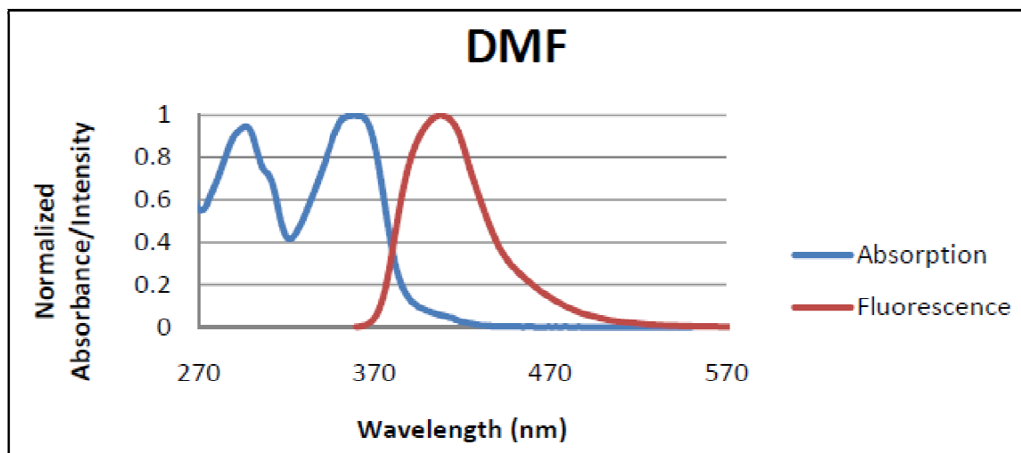
Figure-6: DMF.
