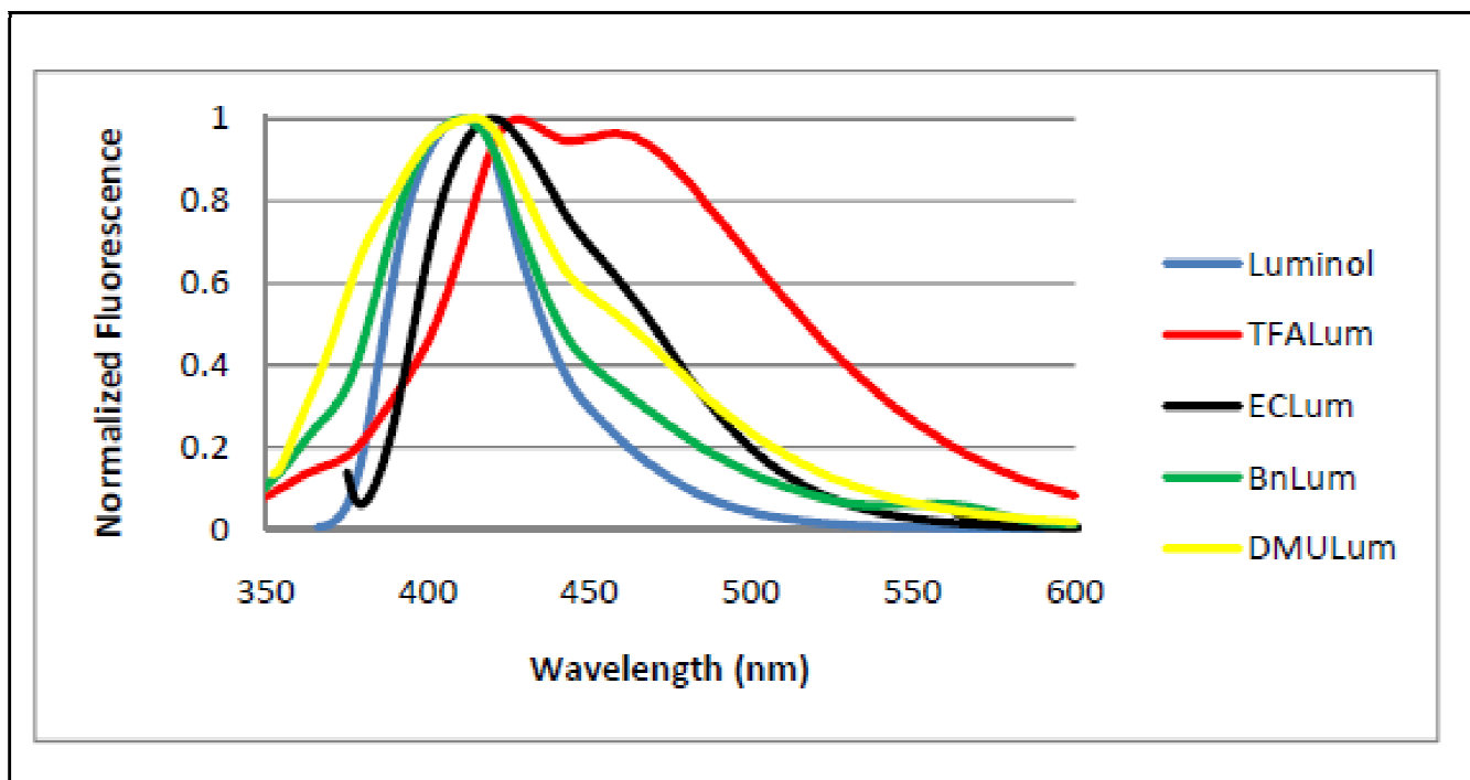
Figure-4: Represent Normalized Fluorescence vs. Wavelength.
