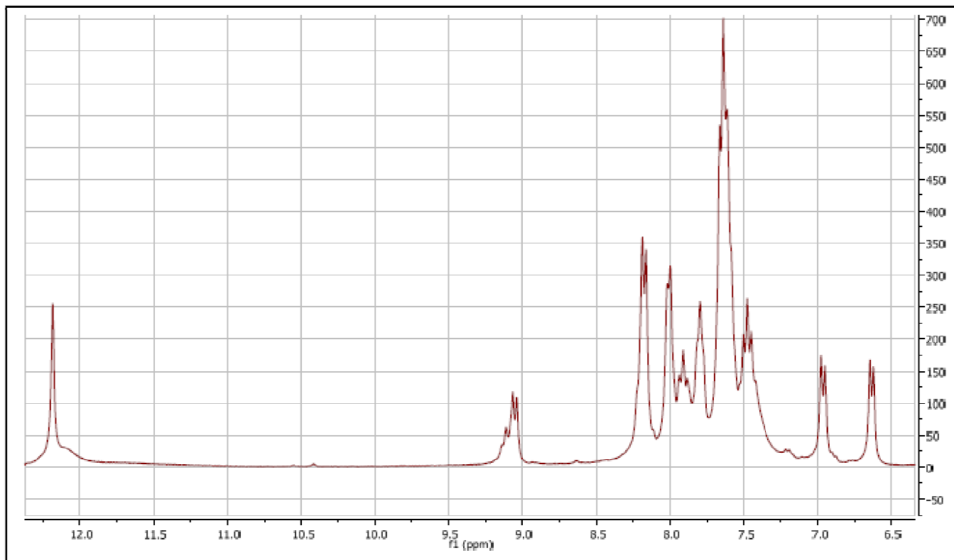
Figure-2: NMR Spectra of bis(2,4,6-tribromophenyl) oxalate (TBPO).
