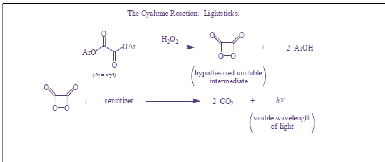
Scheme-2: The Cyalume Reaction: Lightsticks.
