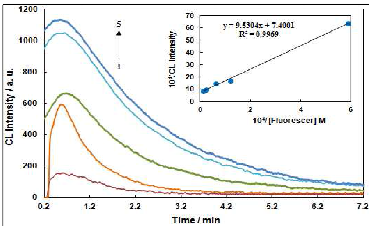
Figure-5: Represent CL underscore vs. fluorescer.
