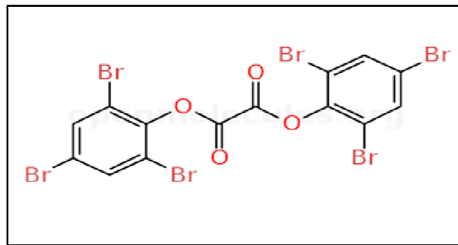
Figure-1 Bis (2,4,6-tribromophenyl) oxalate (TBPO)
